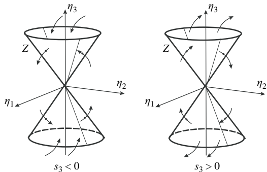
FIGURE 5. Same as figure 3 for the case when \mathbf{M} is indefinite on Z .
