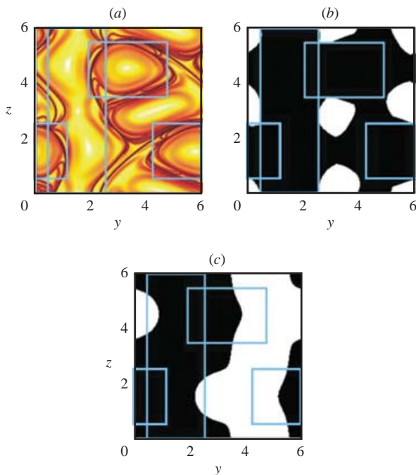
FIGURE 11. The rough location of vortices (marked by rectangles) as inferred from the Lyapunov exponent plot (a), then superimposed on the elliptic region shown in (b), and on the \lambda_2 < 0 region shown in (c).
