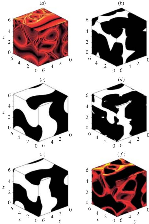
FIGURE 12. Evaluation of different vortex criteria on the faces of the [0, 2\pi]^3 cube in the ABC flow. (a) Finite-time Lyapunov exponents over the time interval [0, 10] , with darker colours indicating higher values. (b) \Delta > 0 (black region). (c) Q > 0 (black region). (d) Q_s > 0 (black region). (e) \lambda_2 < 0 (black region). (f) Time spent in the domain where \mathbf{M}_Z is indefinite, with darker colours indicating larger times.
