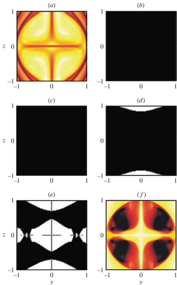
FIGURE 8. Same as figure 7, but with \boldsymbol{\omega} = (0, 0, 3) .
