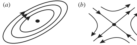
FIGURE 1. Instantaneous streamlines in a z = \text{const.} plane for (a) the velocity field (1.5), (b) the transformed velocity field (1.6).
