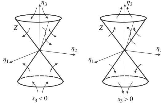
FIGURE 4. Same as figure 3 for the case when \mathbf{M} is positive semidefinite on Z .
