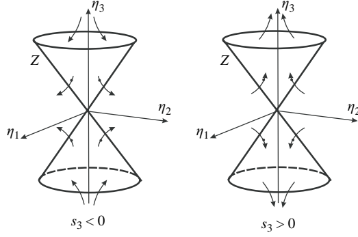
FIGURE 3. Instantaneous flow geometry near the trajectory (now at \eta = 0 ) when \mathbf{M} is positive definite on Z . Dots on the trajectories refer to their point of entry (exit) into (out of) Z .
