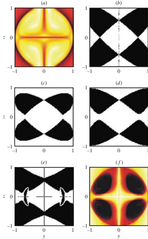
FIGURE 7. Evaluation of different vortex criteria on the (y, z) -plane of the spherical drop flow with \omega = 0 and a = 1 . (a) Finite-time Lyapunov exponents over the time interval [0, 10] , with darker colours indicating higher values. (b) \Delta > 0 (black region). (c) \lambda_2 < 0 (black region). (d) Q > 0 (black region). (e) Q_s > 0 (black region). (f) Time spent in the domain where \mathbf{M}_Z is indefinite, with darker colours indicating longer times.
