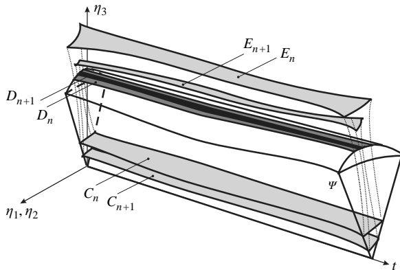
FIGURE 16. The cylinders C_n , D_n , and E_n shown schematically in the four-dimensional space of the (\eta, t) variables.
