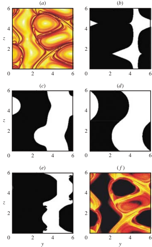
FIGURE 9. Visualization of the intersection of vortices with the x = 2\pi plane in the ABC flow. (a) Finite-time Lyapunov exponents over the time interval [0, 10] , with darker colours indicating higher values. (b) \Delta > 0 (black region). (c) \lambda_2 < 0 (black region). (d) Q > 0 (black region). (e) Q_s > 0 (black region). (f) Time spent in the domain where M_Z is indefinite, with darker colours indicating larger times; if the time is the entire simulation interval [0, 10] , the trajectory is coloured black.
