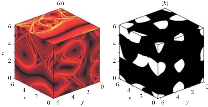
FIGURE 13. (a) Finite-time Lyapunov exponents (with lighter colours indicating larger values) and (b) the elliptic set \mathcal{E} for the ABC flow.
