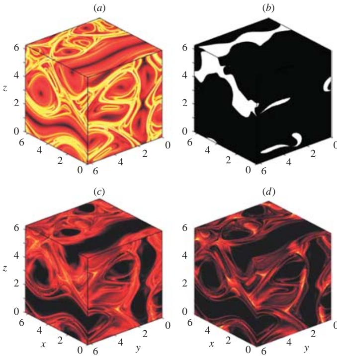
FIGURE 14. Evaluation of different vortex criteria on the faces of the [0, 2\pi]^3 cube in the unsteady ABC-type flow. (a) Finite-time Lyapunov exponents over the time interval [0, 10] , with darker colours indicating higher values. (b) Q_s > 0 (black region). (c) Time spent in the region where \mathbf{M}_Z is indefinite, with darker colours indicating larger times. (d) Time spent in the domain where \mathbf{M} is not positive definite, with darker colours indicating longer times.
