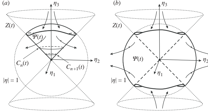
FIGURE 15. The set \Psi(t) for the construction of (a) the stable manifold E^s(t) and (b) the unstable manifold E^u(t) .
