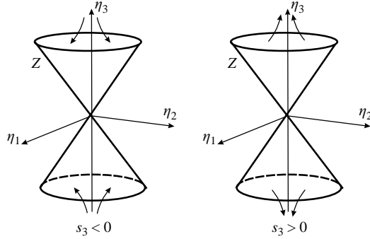
FIGURE 2. The elliptic cone Z in strain basis, and the behaviour of solutions inside Z for s_3 < 0 and s_3 > 0 .
