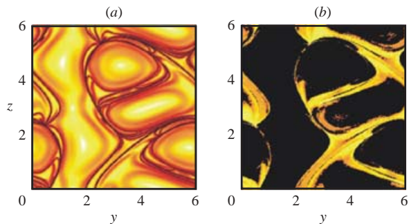
FIGURE 10. Visualization of the intersection of vortices with the x = 2\pi plane in the ABC flow. (a) Finite-time Lyapunov exponents over the time interval [0, 10] , with darker colours indicating higher values. (b) Time spent in the domain where M_Z is indefinite; if the time is at least 90% of the entire simulation interval [0, 10] , the trajectory is coloured black.
