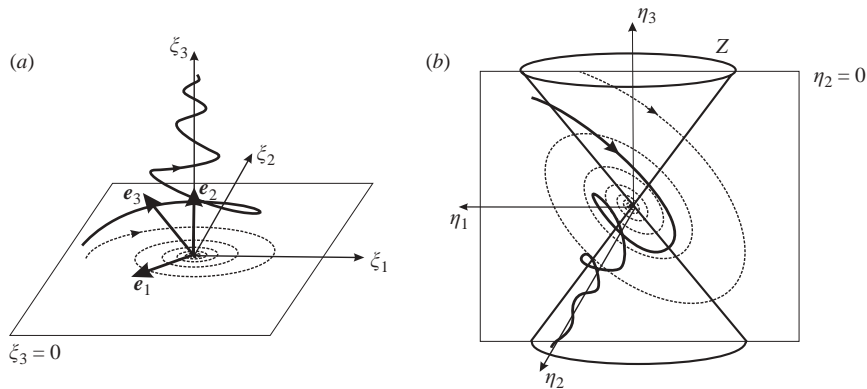
FIGURE 6. The linearized flow generated by the velocity gradient (4.3): (a) in the original basis (b) in strain basis.
